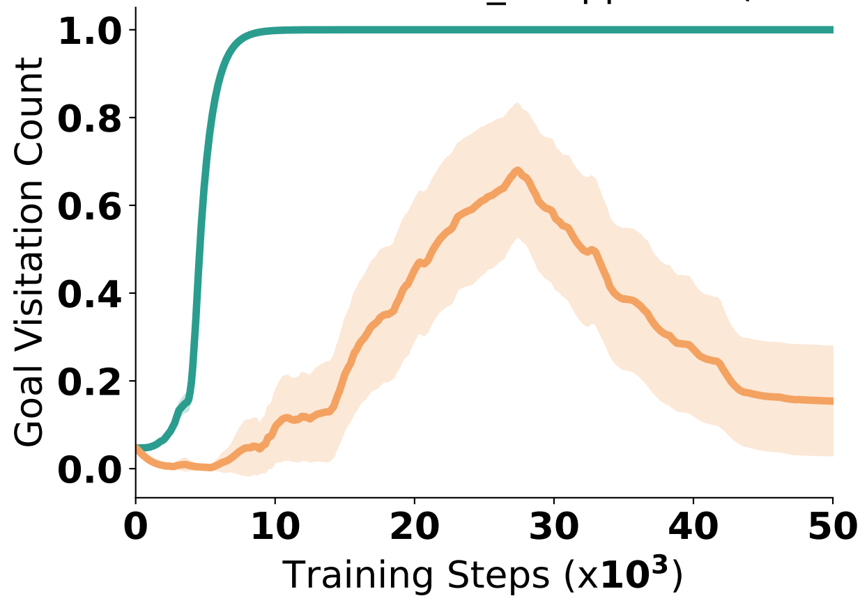
Gridworld-Bottleneck_NSupporters(100%)
